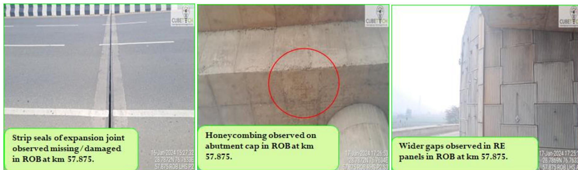
Figure 4-2: Condition of ROB
