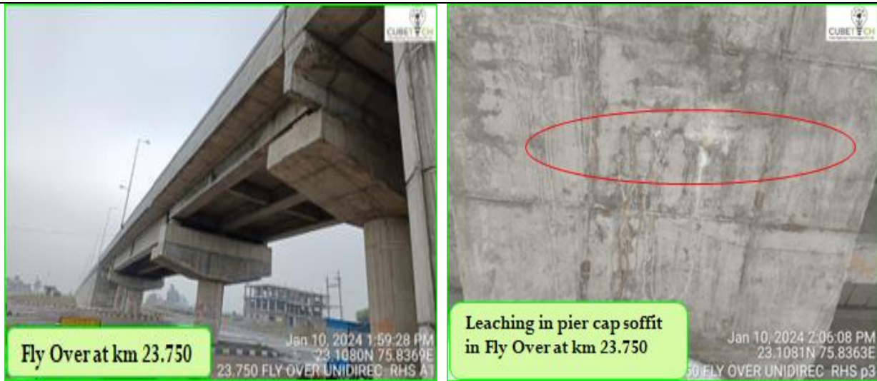
Figure 4-3: Condition of Flyovers
