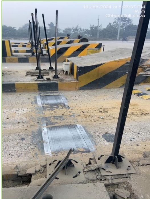
Figure 3-18: Medium Speed Weigh in Motion (MSWIM).
